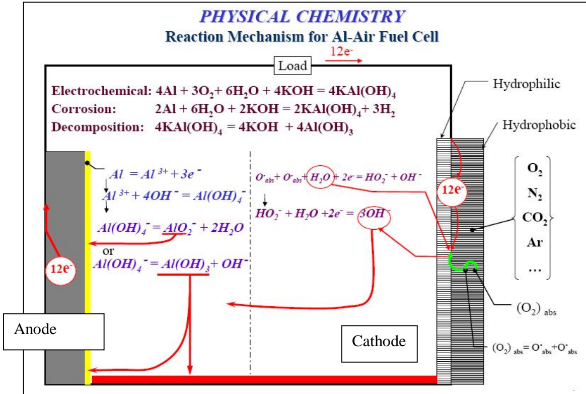
Fig. 1. Reaction mechanisms for aluminum-air fuel cell
