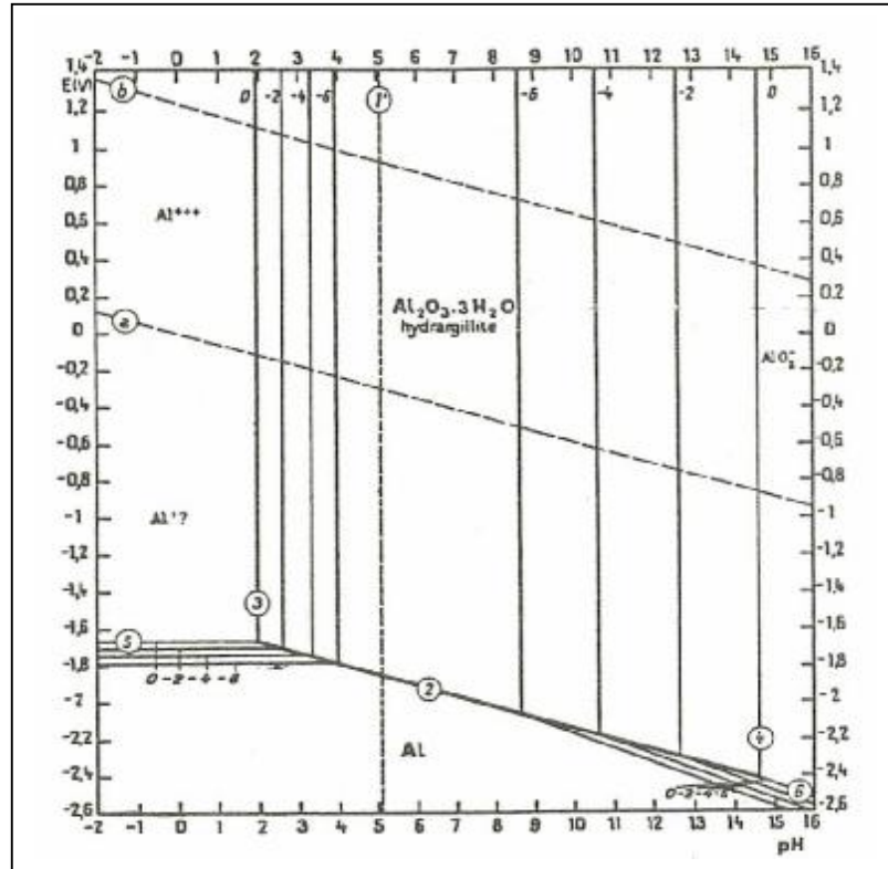
FIG. 1 Pourbaix Diagrams and Reactions of Aluminum-Water system
