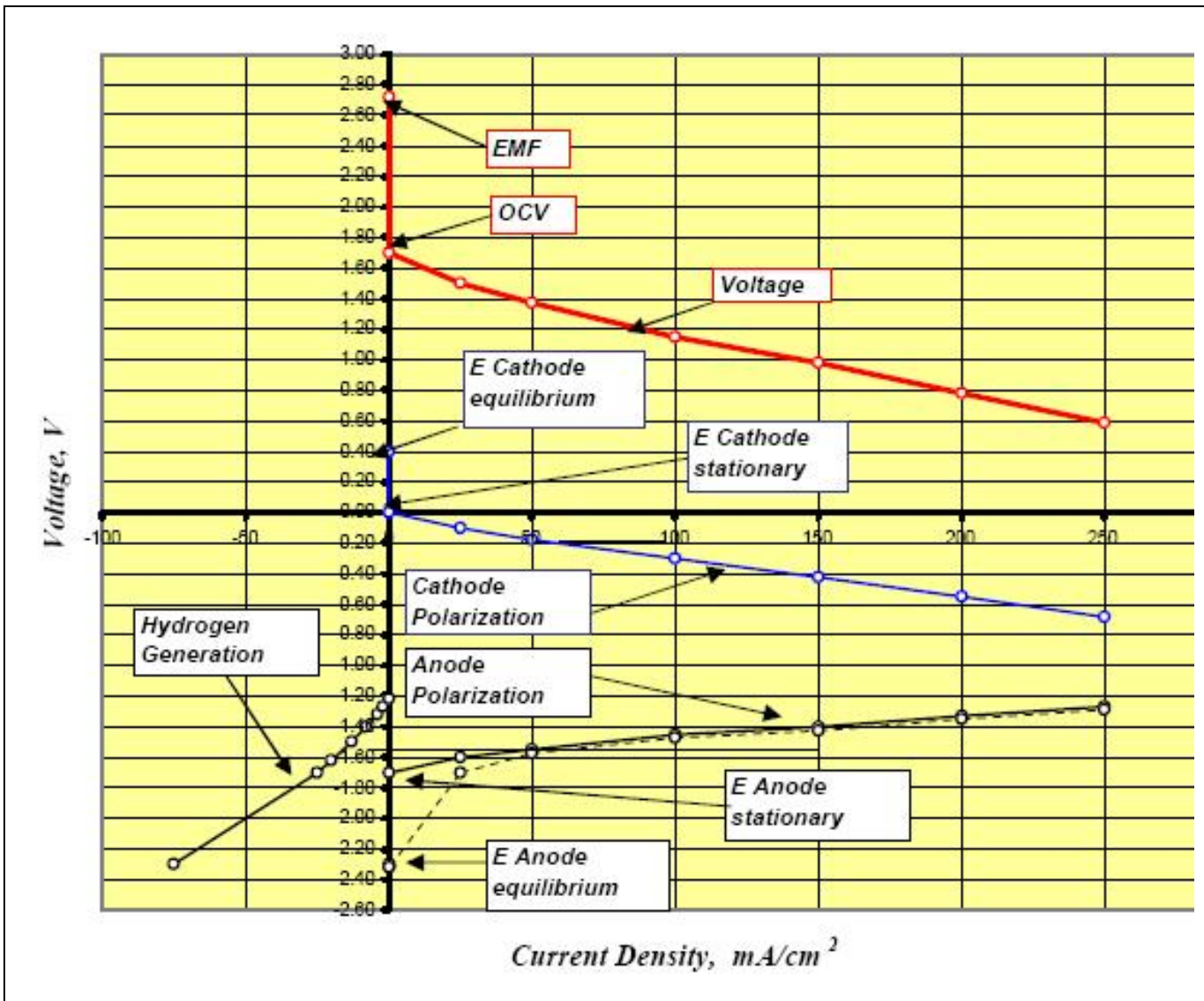
Fig. 2. Voltage vs. Current density diagram of aluminum-air fuel cell
